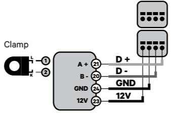
N1 CT
