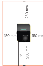
I-1: Mounting area
